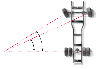
Toe-out on turn
