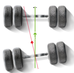
Thrust Angle
